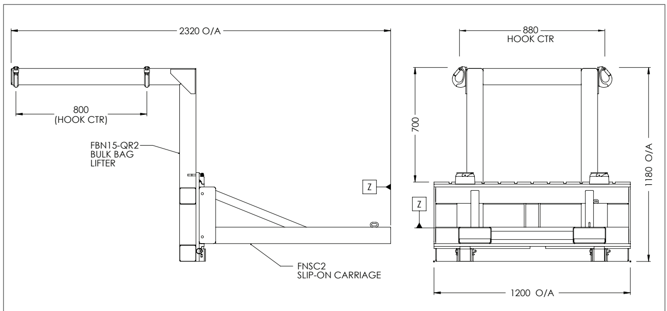
Slip-on Carriage allows attachment to be connected to the forks of a forklift
